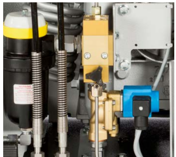
Time saving through automatic operation of the compressor: automatic condensate drain system mounted on a MARINER 250.
