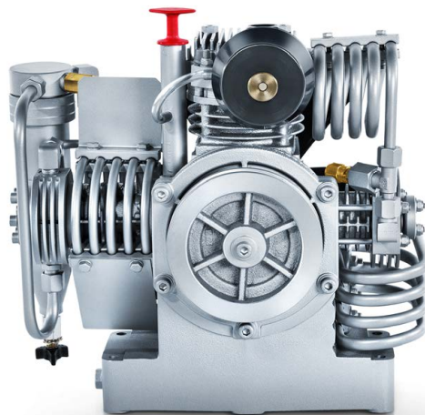
OCEANUS Compressor Block
